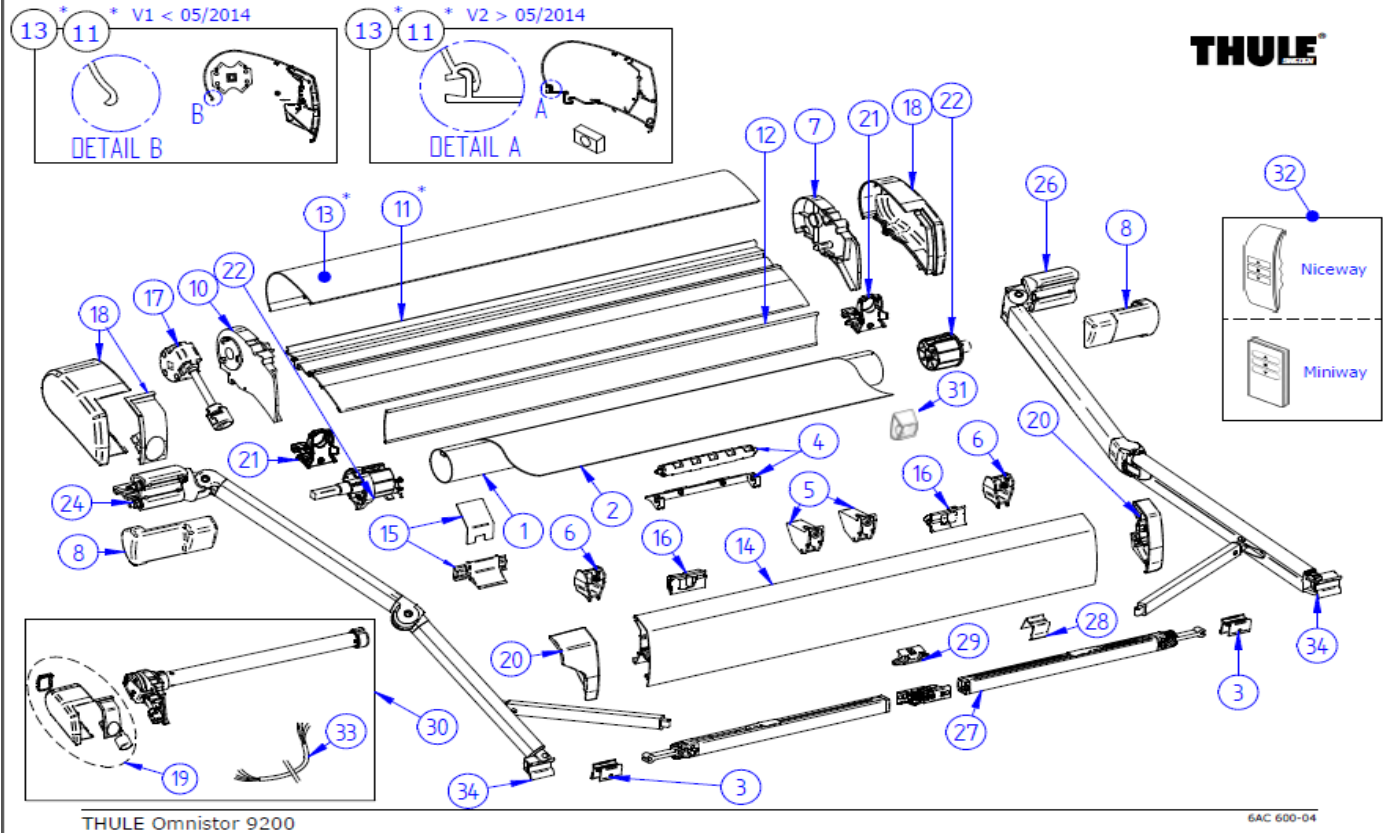
THULE Omnistor 9200
