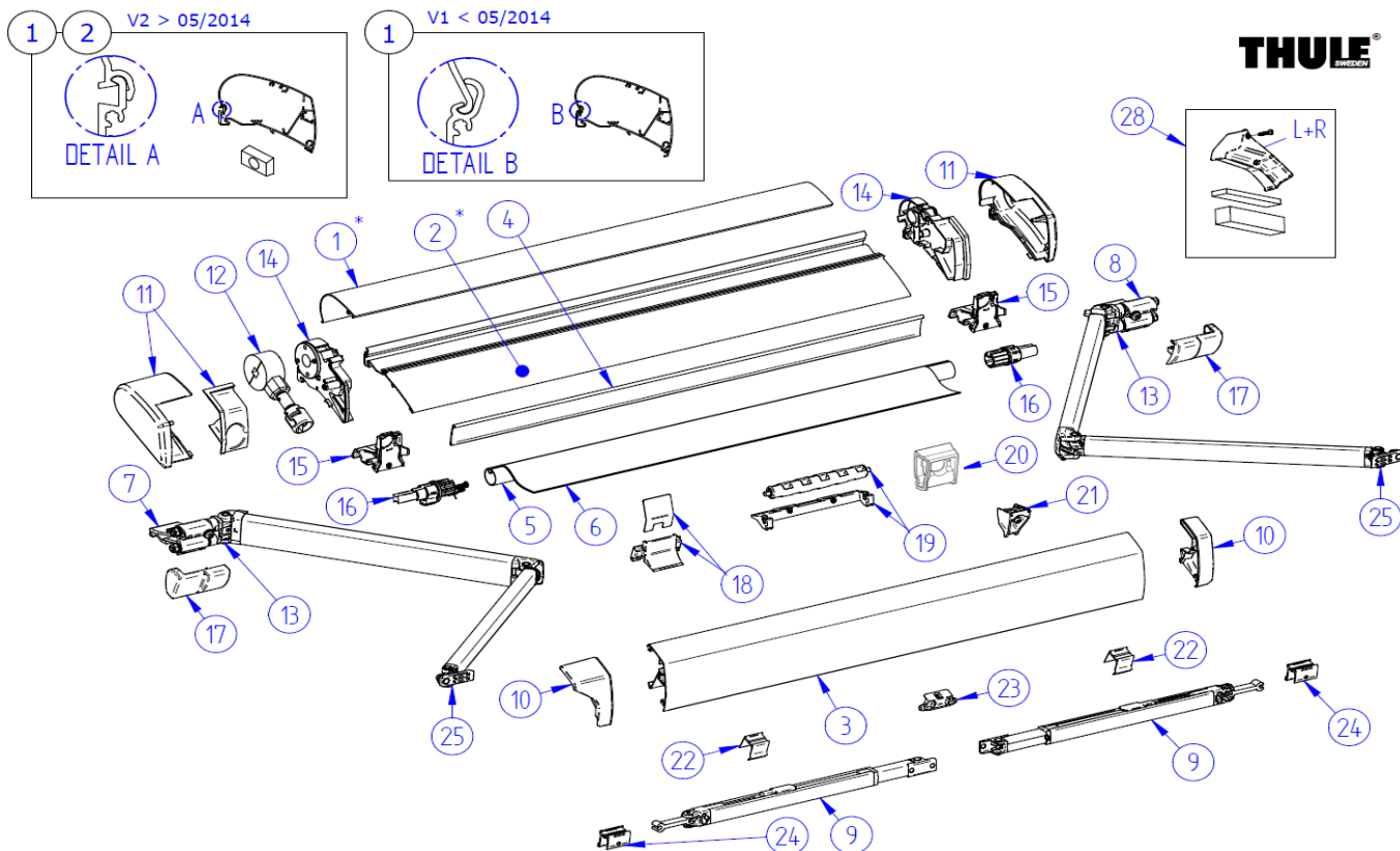
THULE Omnistor 6200
