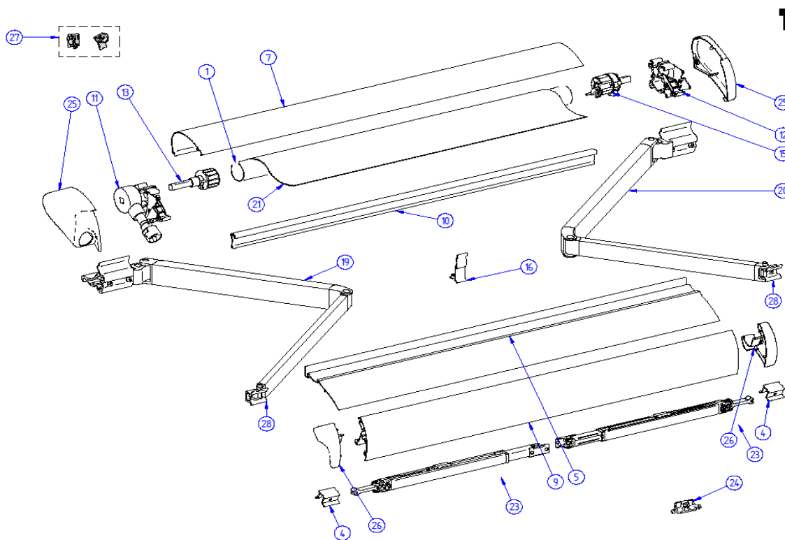
THULE Omnistor 6002
